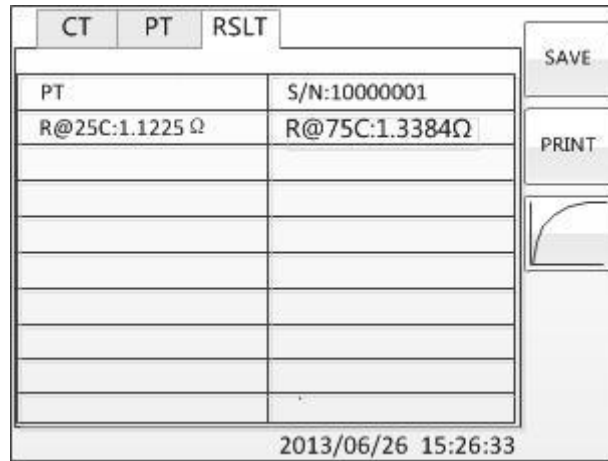
Fig 8 PT's test results interface
