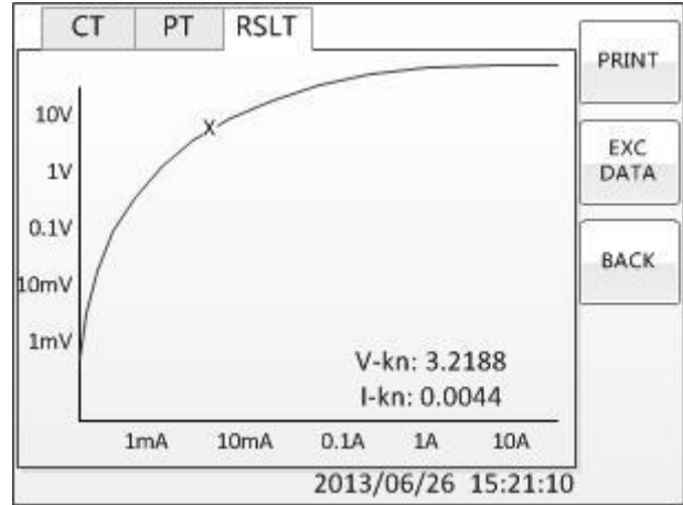
Fig 16 Excitation curve interface
