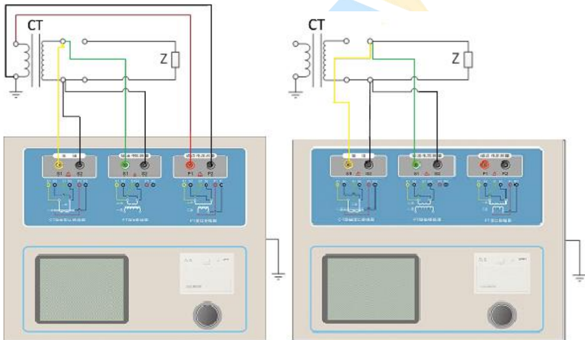
Fig 1 DC resistance, excitation, ratio experiment connection
