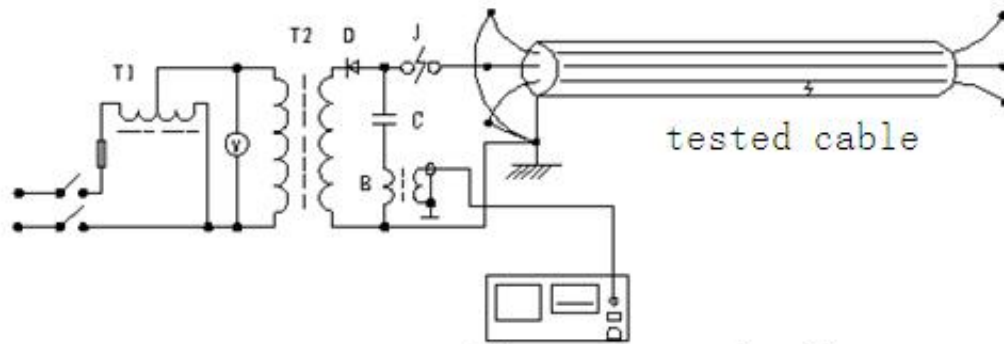
current sampling schematic diagram by impulse HV flash-over method
