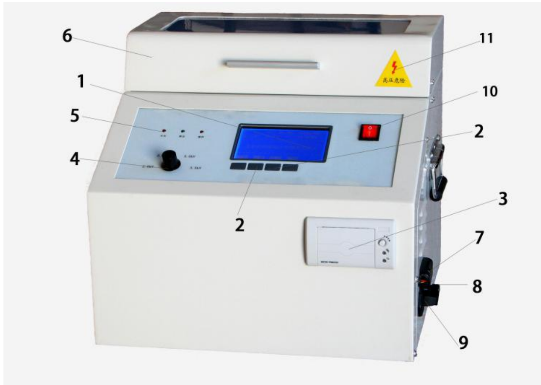
ZXJYD-I Insulating Oil Breakdown Voltage Tester
